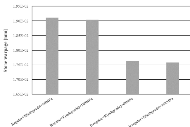
Figure 12. Stone warpage of the pavements.
