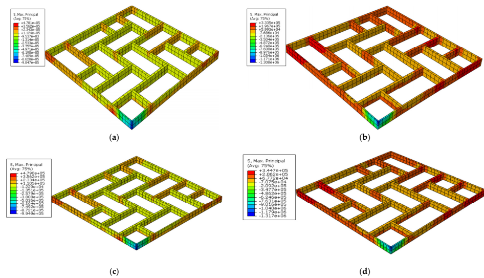
Figure 9. Maximum principal stress distribution in the mortar joints: (a) H-SPS + E (subgrade = 180 MPa), (b) R-SPS + E (subgrade = 180 MPa), (c) H-SPS + E (subgrade = 60 MPa), (d) R-SPS + E (subgrade = 60 MPa).
