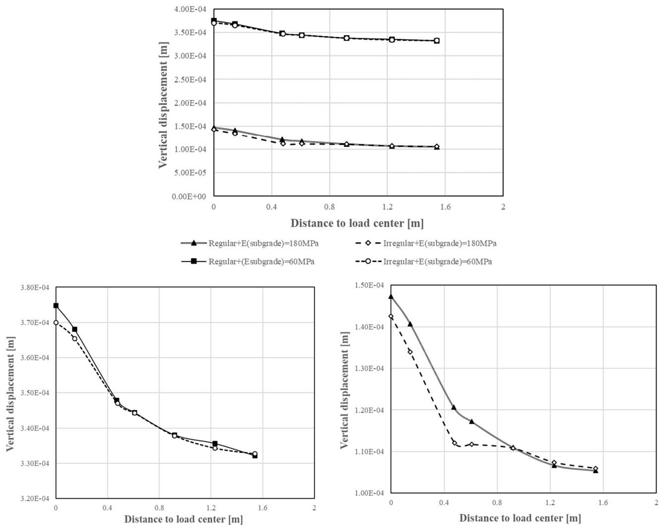
Figure 8. Vertical displacement for the R-SPS and H-SPS.
