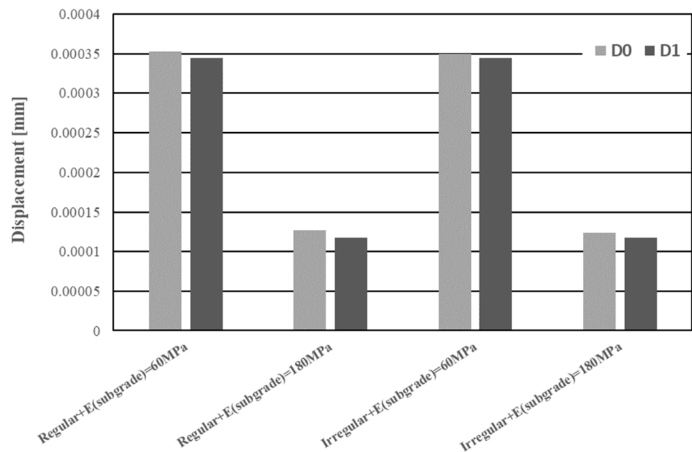
Figure 16. Displacements at the two points next to the joint.
