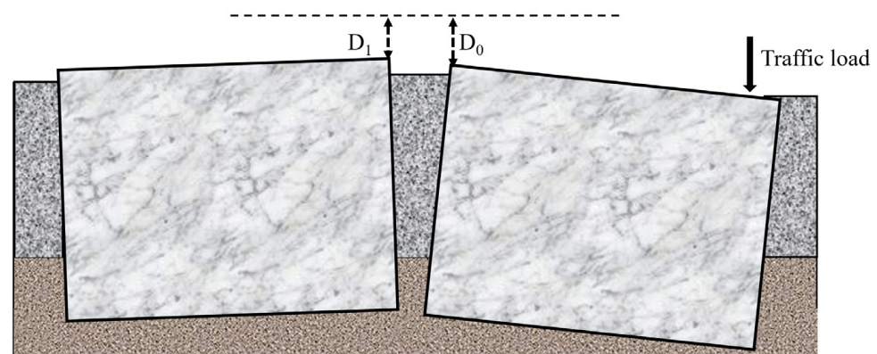
Figure 15. Joint efficiency characterized by the LTE.
