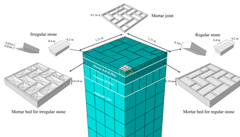
Figure 7. Physical model sizes and FEM mesh.
