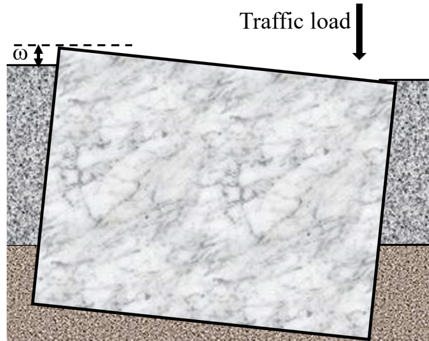
Figure 13. Separation behavior between the mortar joint and stone.
