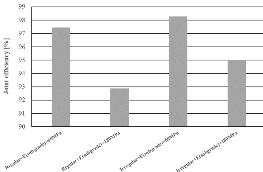
Figure 17. Joint efficiency for the pavements.
