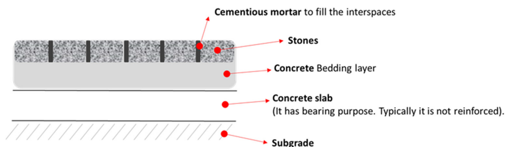
Figure 2. Cross-section of a SPS (this structure is similar to the one considered as a case study in the present research).
