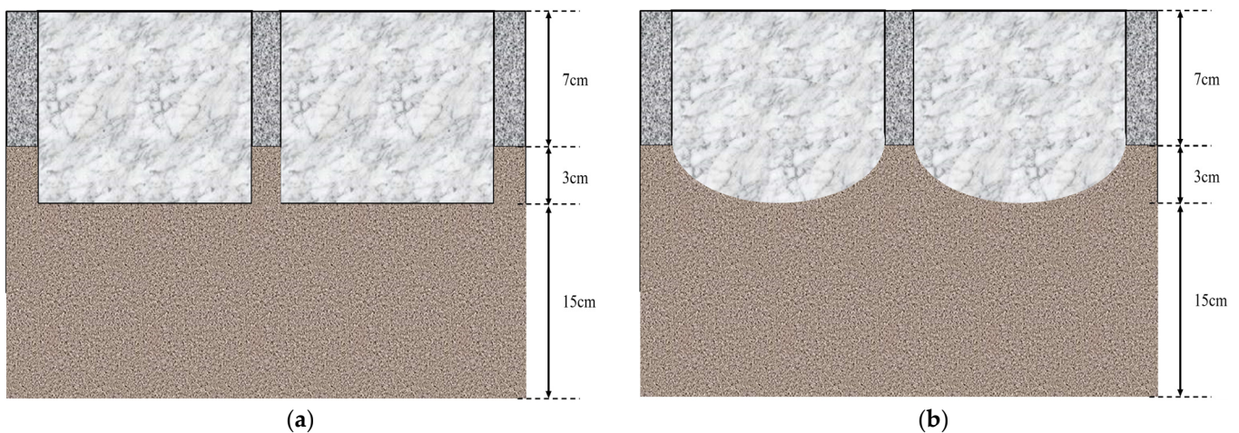
Figure 6. The geometry of SPS; (a) R-SPS, (b) H-SPS.
